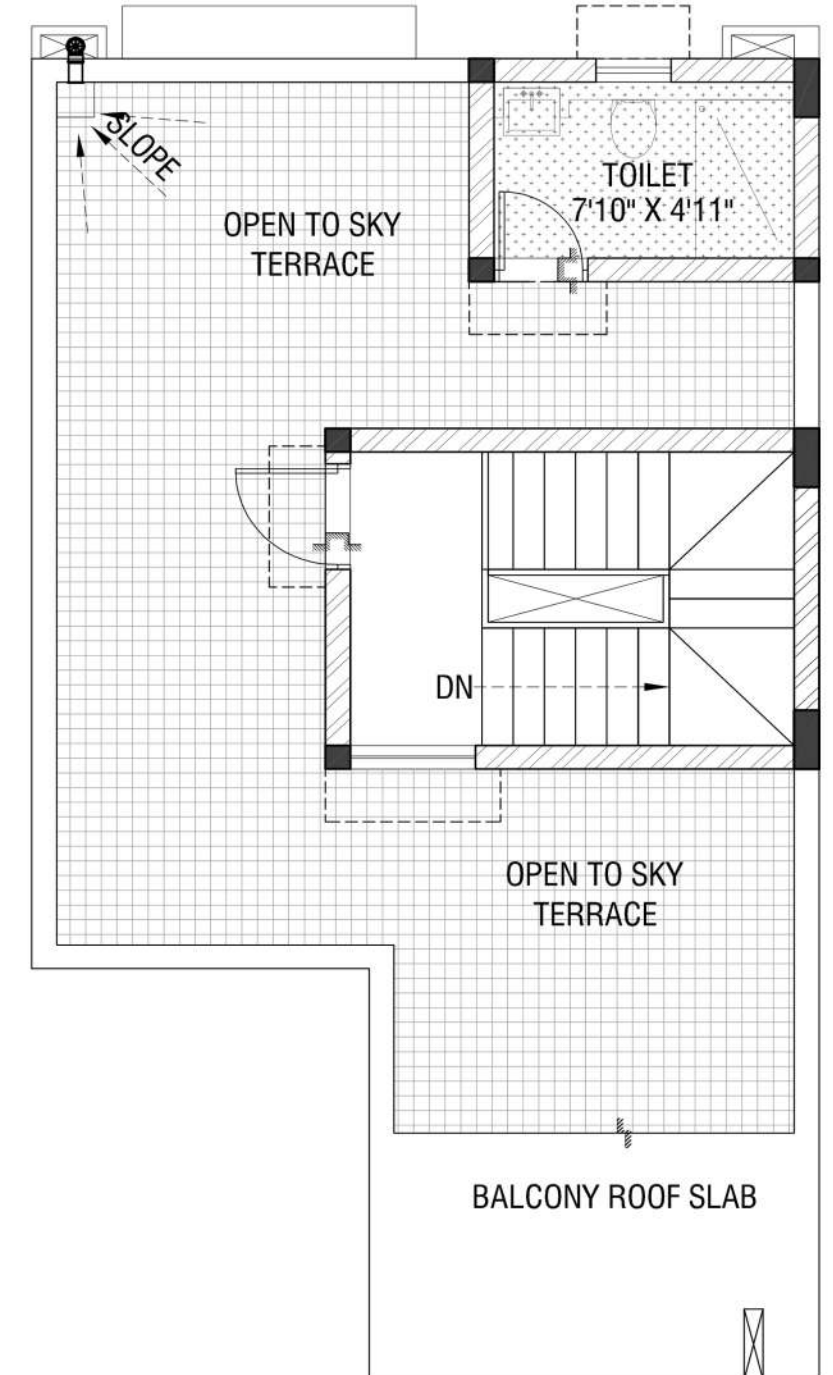
Roof Plan
