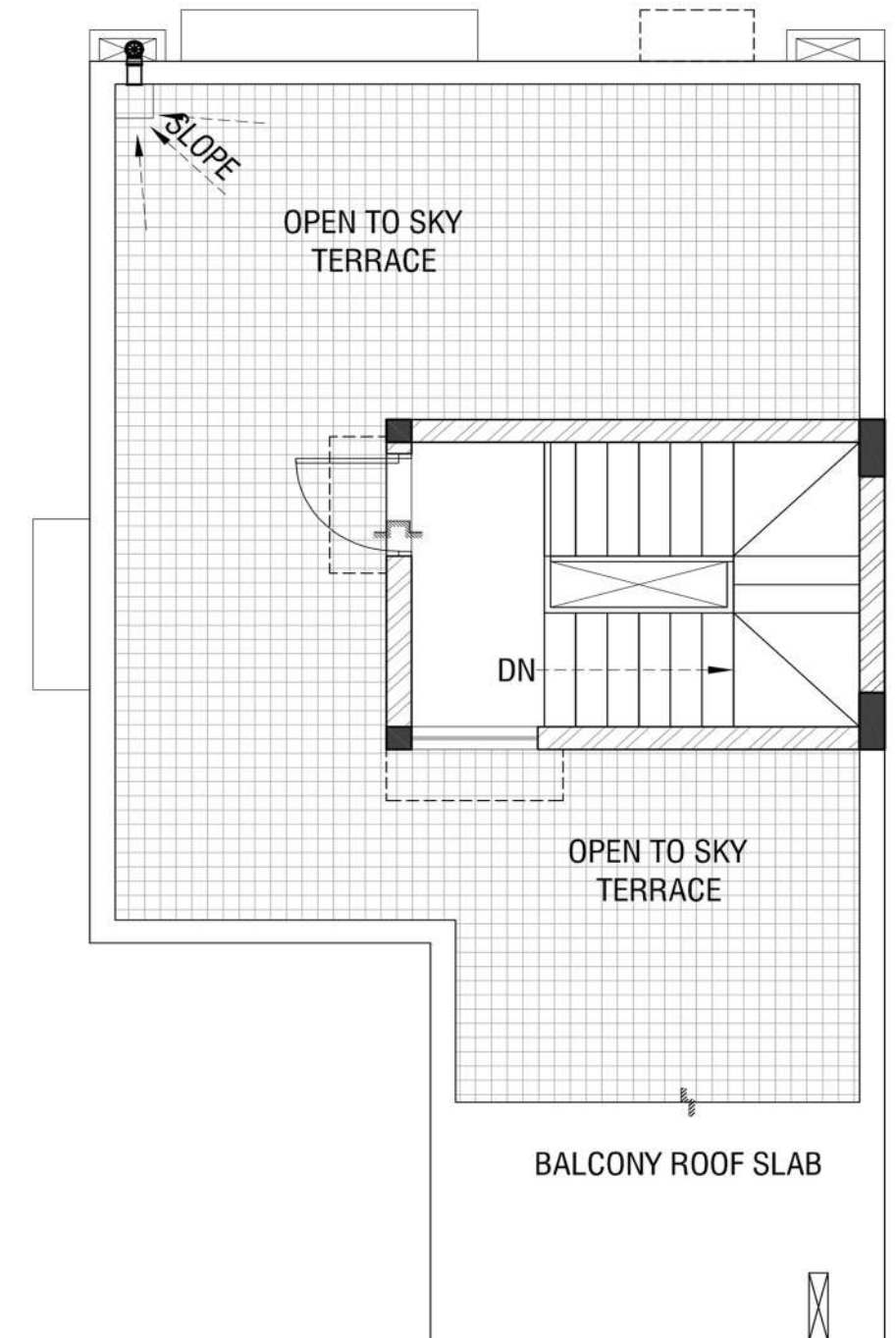
Roof Plan
