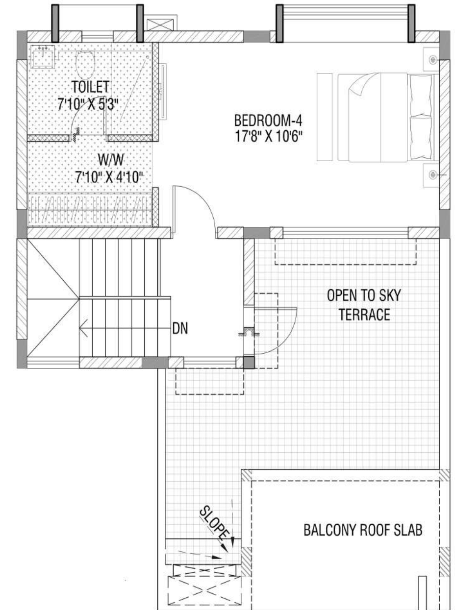
Roof Plan
